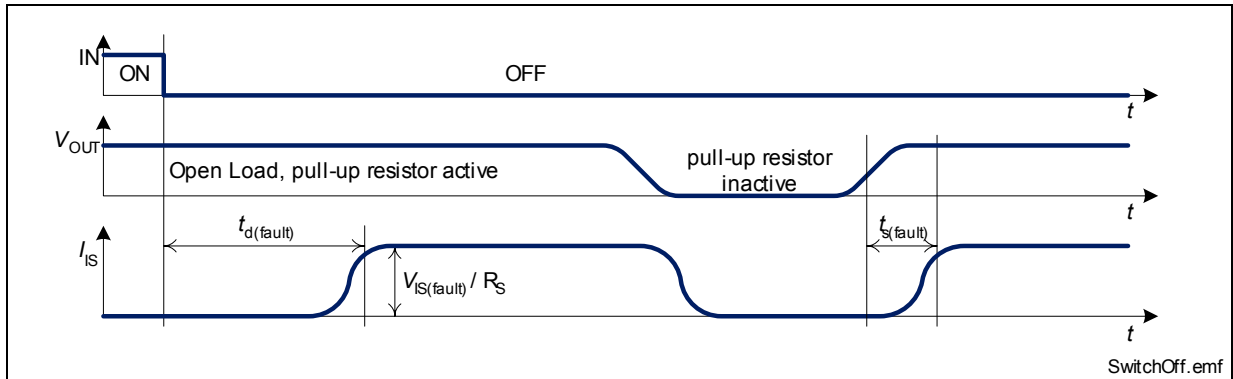
Figure 17 Timing of Diagnosis Signal in OFF-state
