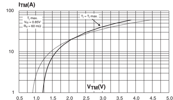
Figure 4: On-state characteristics (maximum values)
