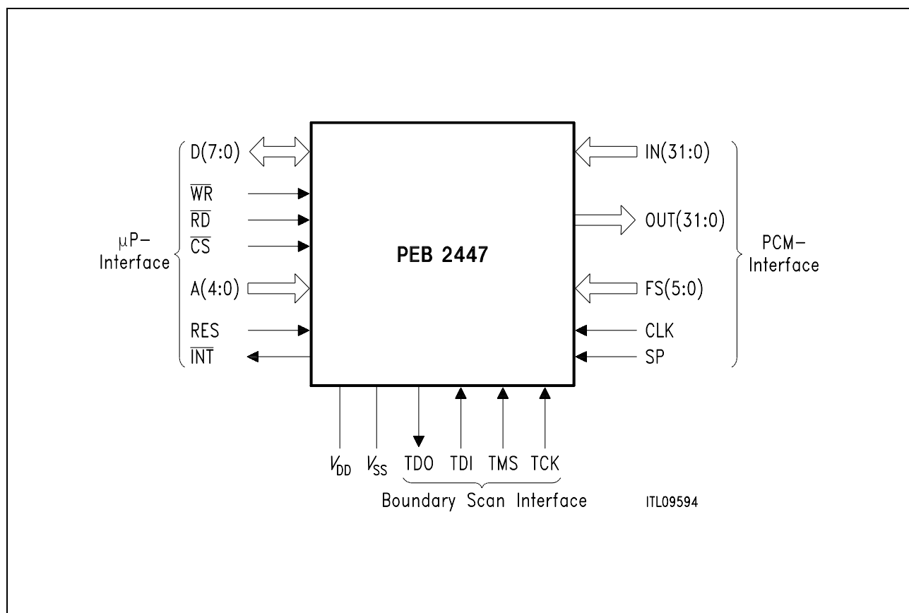
Figure 1 Functional Symbol
