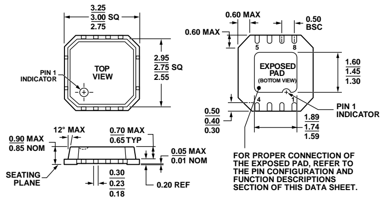
Figure 26. 8-Lead Lead Frame Chip Scale Package [LFCSP_VD] 3 mm x 3 mm Body, Very Thin, Dual Lead (CP-8-2) Dimensions shown in millimeters
