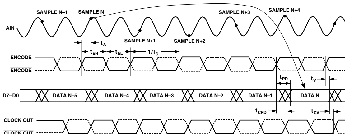
Figure 1. Timing—Single Channel Mode
