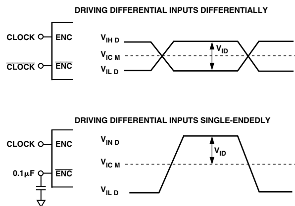
Figure 10. Input Signal Level Definitions
