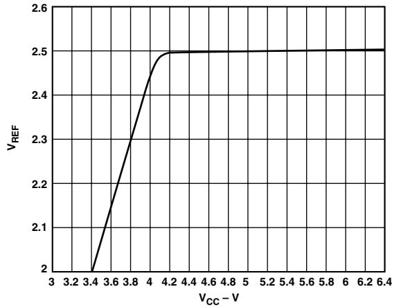
TPC 5. Reference Voltage vs. Power Supply Voltage
