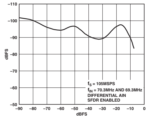
TPC 24. Third Order IMD vs. AIN Level, f_S = 105 MSPS, f_{IN} = 70.3 MHz and 69.3 MHz, Differential AIN, SFDR Enabled
