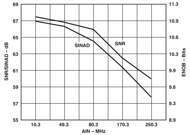
TPC 10. SNR and SINAD vs. AIN Frequency. Differential AIN @ -0.50 dBFS, f_S = 125 MSPS, SFDR Enabled
