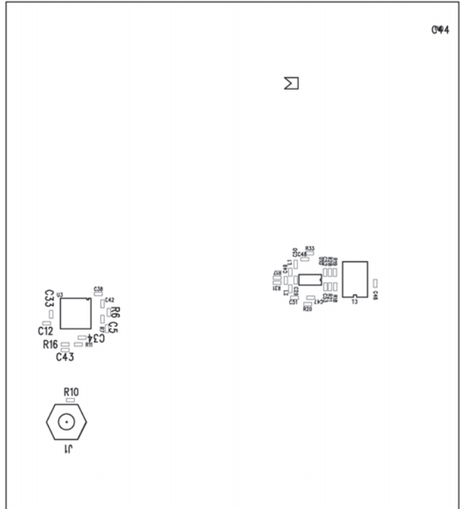
Figure 21. Bottom Silkscreen
