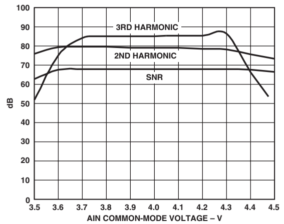
TPC 11. Dynamic Performance vs. AIN Common-Mode Voltage. Differential AIN @ -0.5 dBFS, f_{IN} = 49.3 MHz, f_S = 105 MSPS
