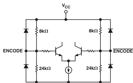
Figure 5. Encode Inputs
