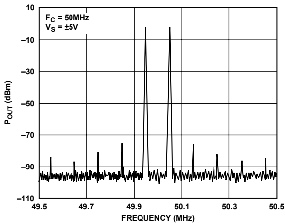
Figure 19. Intermodulation Distortion
