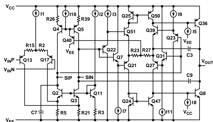
Figure 34. AD8044 Simplified Schematic
