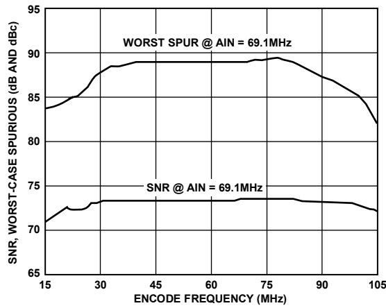
Figure 21. SNR, Worst-Case Spurious vs. Encode @ 69.1 MHz
