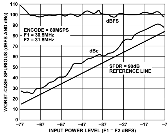
Figure 17. Two-Tone SFDR @ 30.5 MHz and 31.5 MHz
