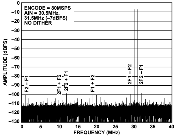
Figure 16. Two-Tone SFDR @ 30.5 MHz and 31.5 MHz
