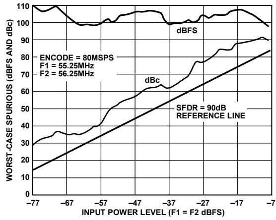
Figure 20. Two-Tone SFDR @ 55.25 MHz and 56.25 MHz
