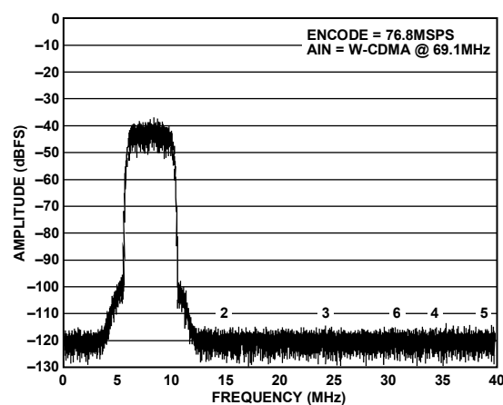
Figure 27. W-CDMA Tone @ 69.1 MHz, Encode = 76.8 MSPS
