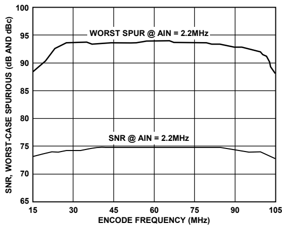
Figure 18. SNR, Worst-Case Spurious vs. Encode @ 2.2 MHz
