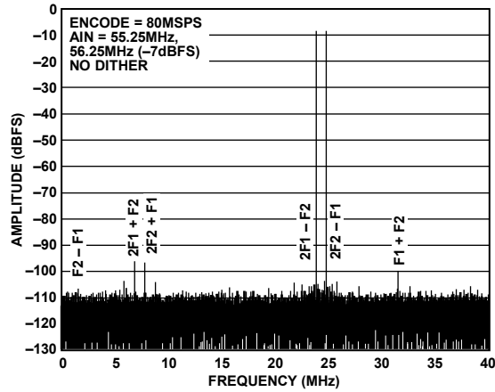
Figure 19. Two-Tone SFDR @ 55.25 MHz and 56.25 MHz
