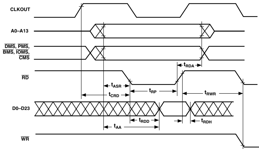
Figure 24. Memory Read
