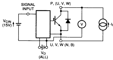
Figure 3 V EC Test
