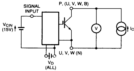
Figure 1 V CES Test
