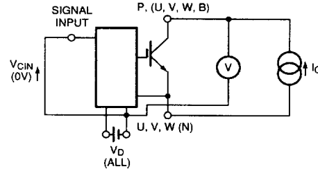
Figure 2 V CE(SAT) Test
