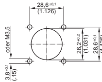
Panel cutout
