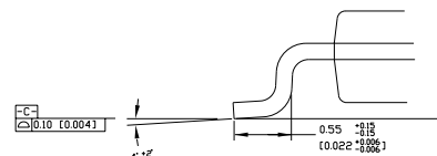
DETAIL A
