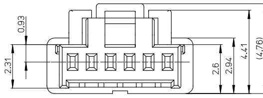
VIEW "D"
