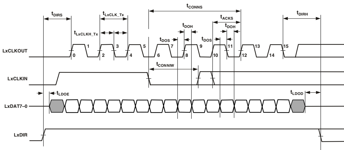
Figure 16. Link Ports—Transmit
