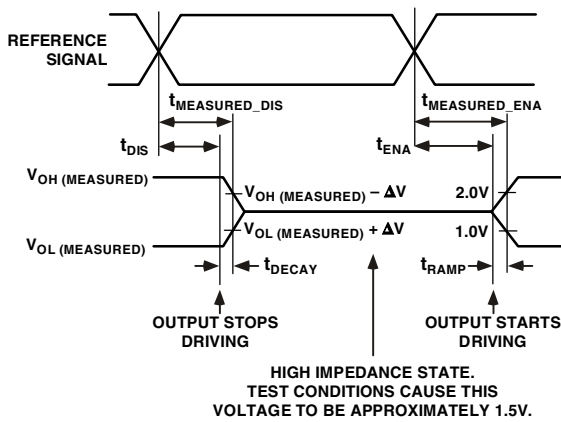
Figure 29. Output Enable/Disable
