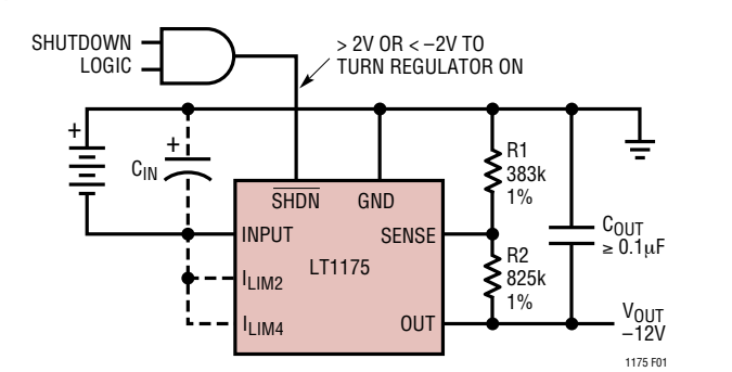
Figure 1. Typical LT1175 Adjustable Connection
