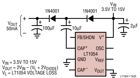
Positive Doubler
