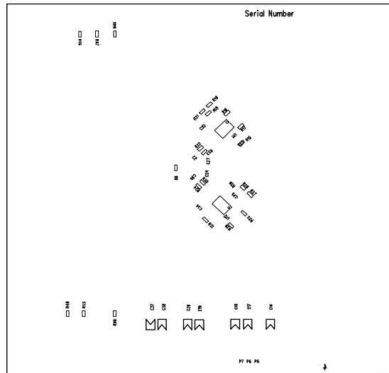
Figure 52. Bottom Silkscreen
