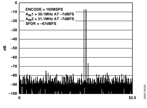
Figure 24. Two-Tone Intermodulation Distortion (30 MHz and 31 MHz; 1 V p-p, FS = 105 MSPS)
