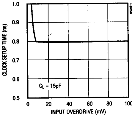
CLOCK SETUP TIME vs. INPUT OVERDRIVE
