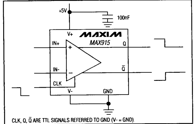
Figure 3. Single-Supply Operation
