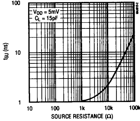
CLOCK SETUP TIME vs. SOURCE RESISTANCE
