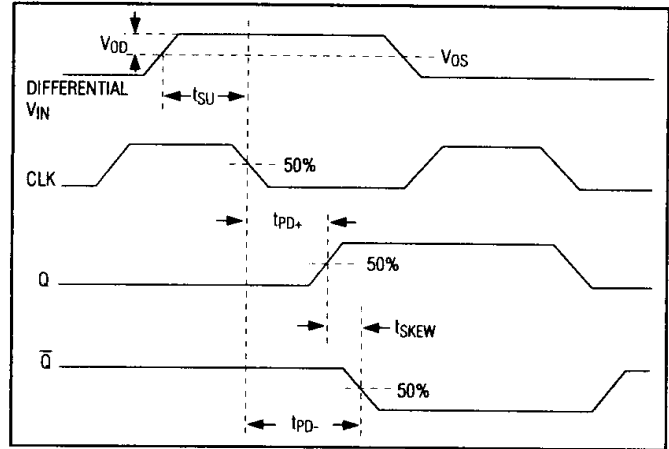
Figure 1. Timing Diagram
