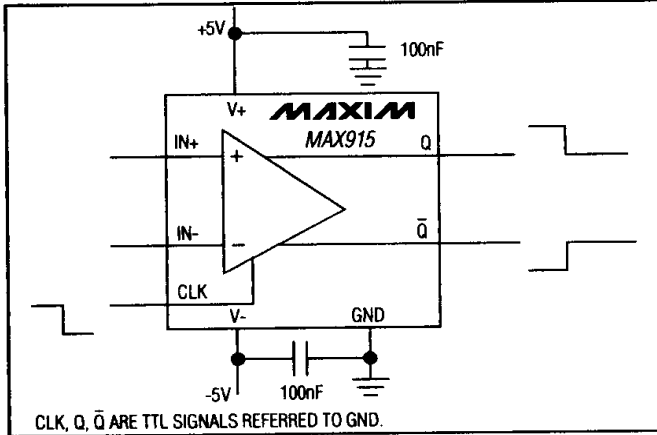
Figure 2. Dual-Supply Operation
