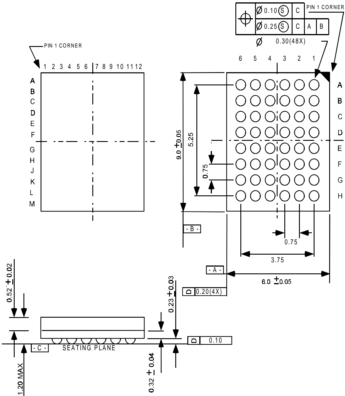
TOP VIEW
