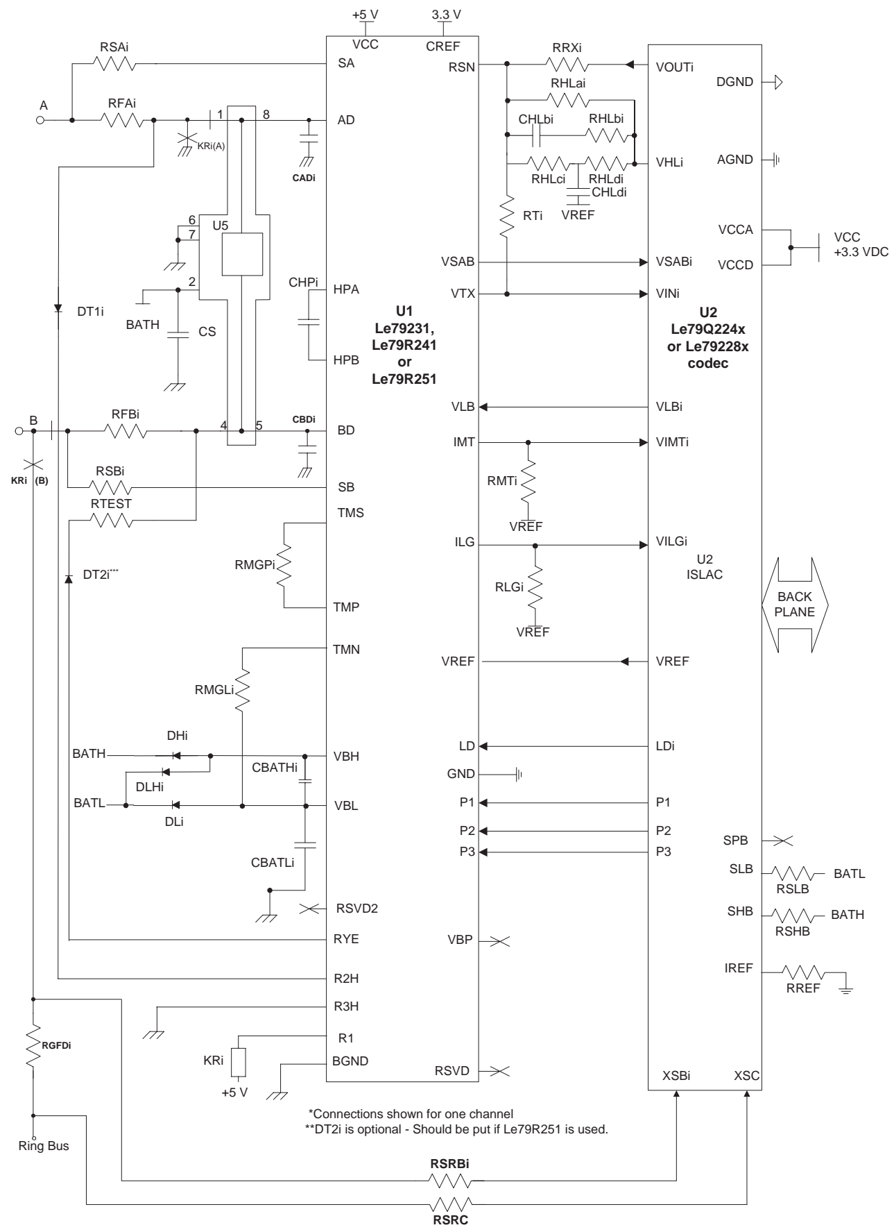
Figure 6. External Ringing Line Schematic
