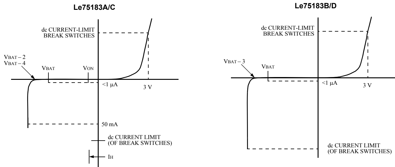
Figure 3. Protection Circuits
