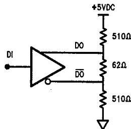
25 MBS Driver Propagation Delay Test Circuit
