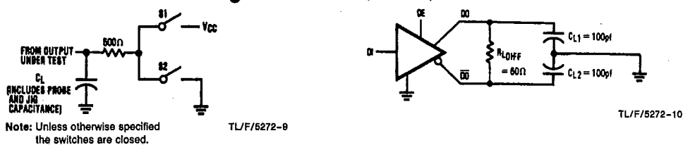
FIGURE 4. Driver Propagation Delay Test Circuits
