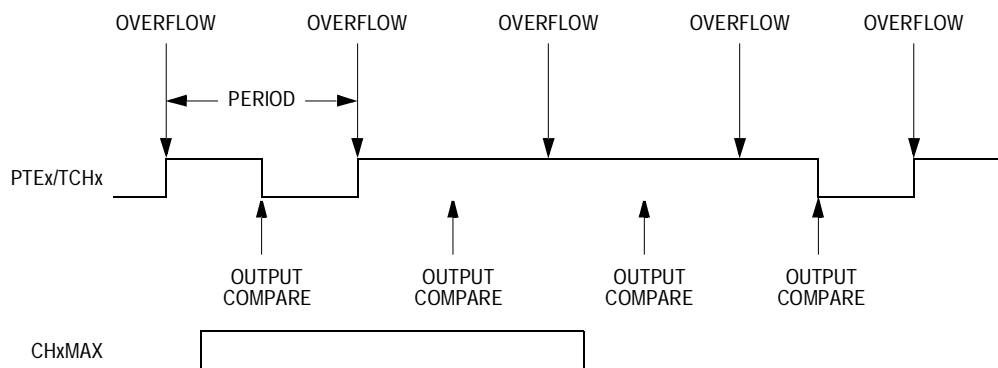
Figure 22-8. CHxMAX Latency
