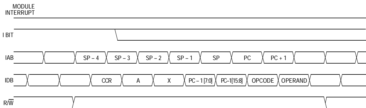
Figure 9-9. Interrupt Recovery
