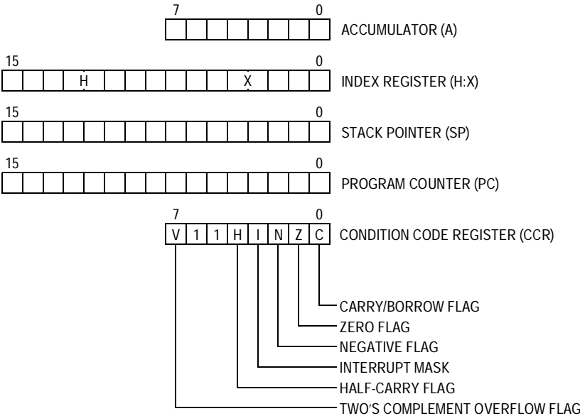
Figure 8-1. CPU Registers
