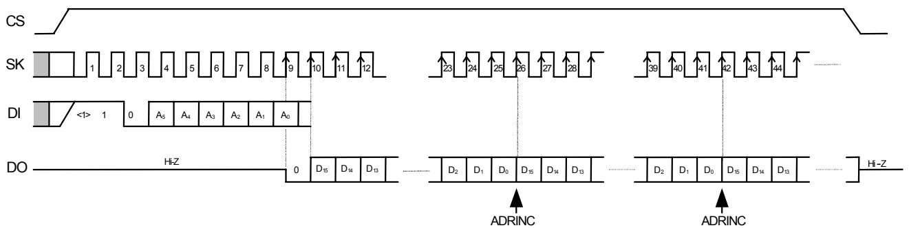
Figure 7 Read Timing (S-93C46B)
