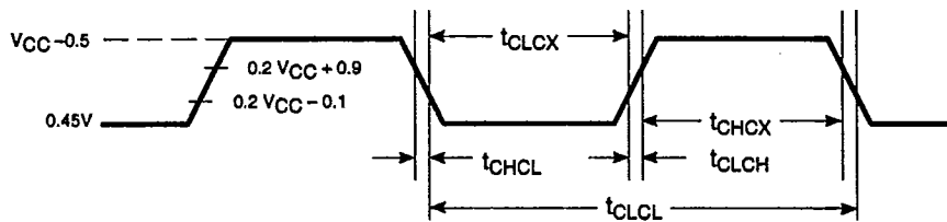
Figure 1. External Clock Drive
