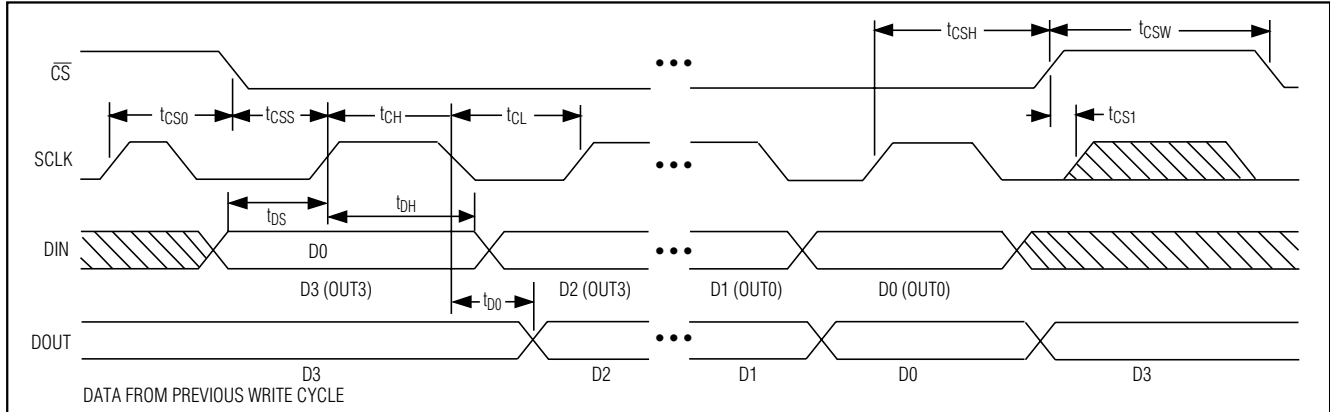
Figure 6. Serial-Mode Timing
