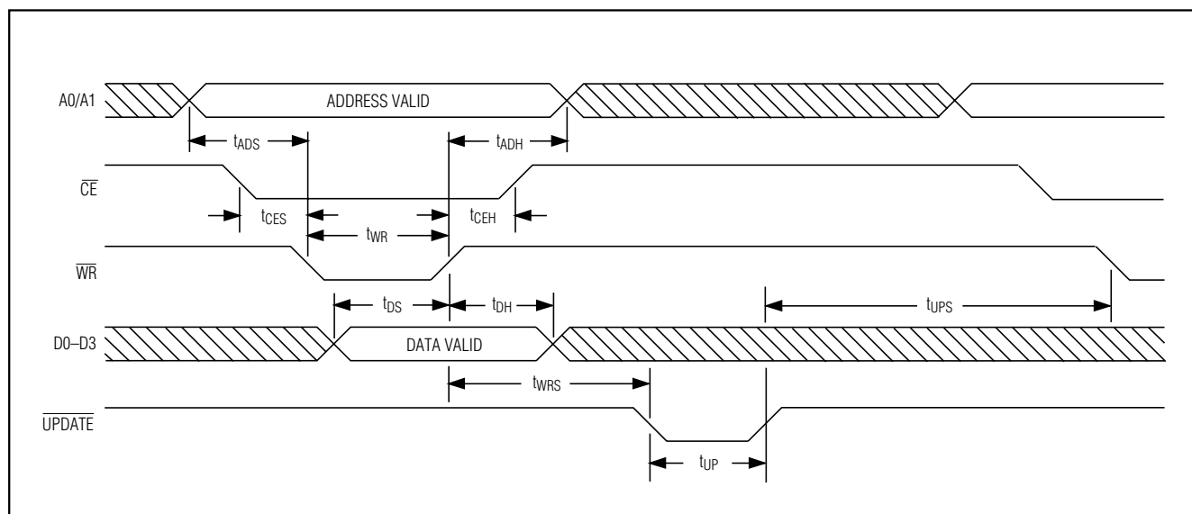
Figure 4. Parallel-Mode Timing
