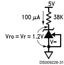
FIGURE 3. 1.2V Reference
