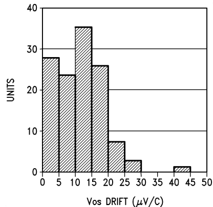
Average V_{OS} Drift Industrial Temperature Range
