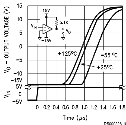
Comparator Response Times—Non-Inverting Input, Positive Transition
