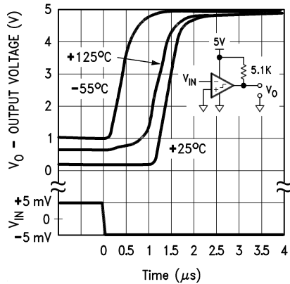
Comparator Response Times—Inverting Input, Positive Transition
