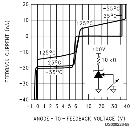
FEEDBACK Current vs FEEDBACK-to-Anode Voltage
