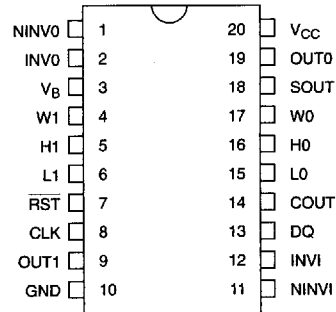
20-Pin DIP (300 Mil) and 20-Pin SOIC See Mech. Drawings Section
