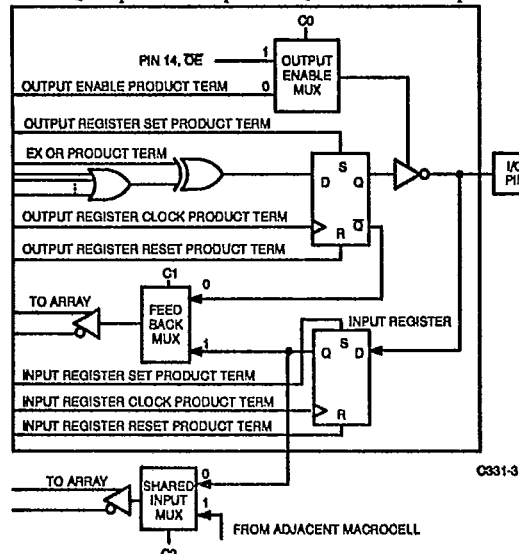
Figure 1. I/O Macrocell
