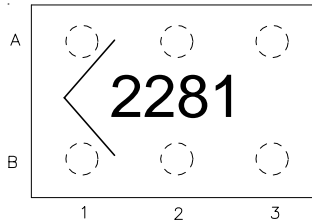
3 x 2 Grid Flip Chip TVS (Top View)
