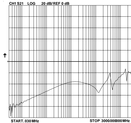
Analog Crosstalk (B1 to A3)
