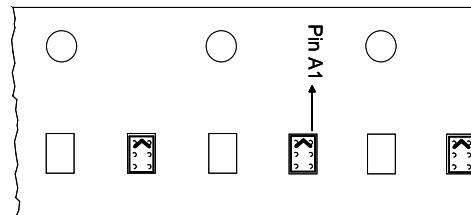
Device Orientation 2mm pitch option (All pockets populated)
