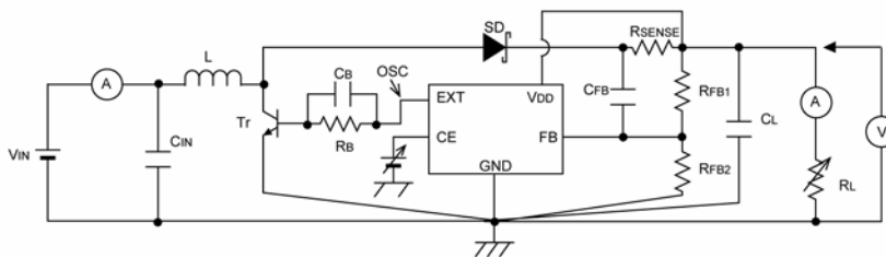
Circuit
