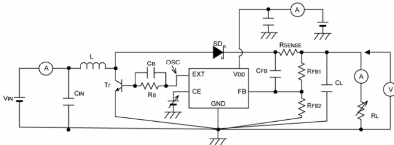
Circuit
