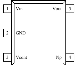
TK707xxS (SOT23-5)
