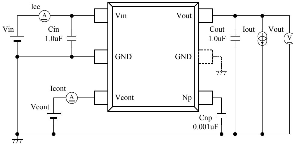
TK708xxH (SON2017-6)
