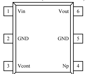
TK708xxH (SON2017-6)
