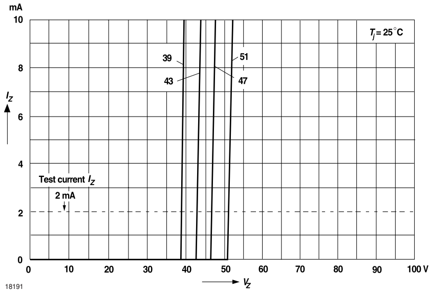
Figure 18. Breakdown Characteristics
