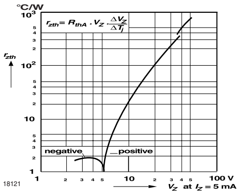
Figure 8. Thermal differential resistance versus Zener voltage
