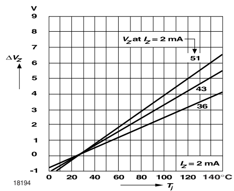
Figure 12. Change of Zener voltage versus junction temperature
