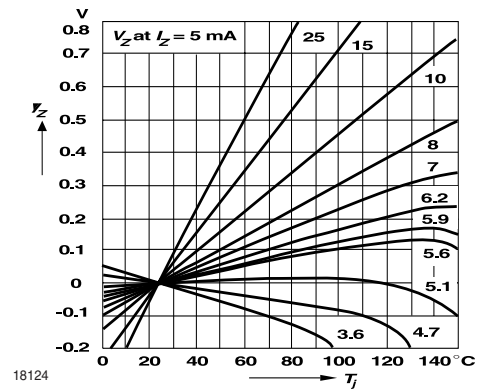
Figure 11. Change of Zener voltage versus junction temperature
