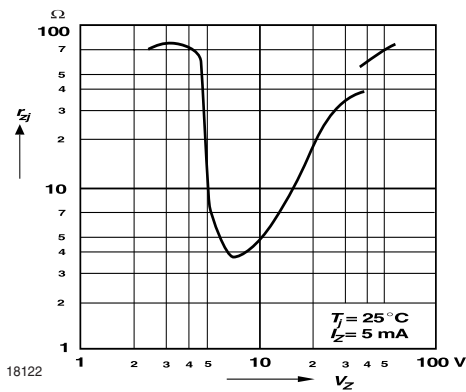
Figure 9. Dynamic resistance versus Zener voltage
