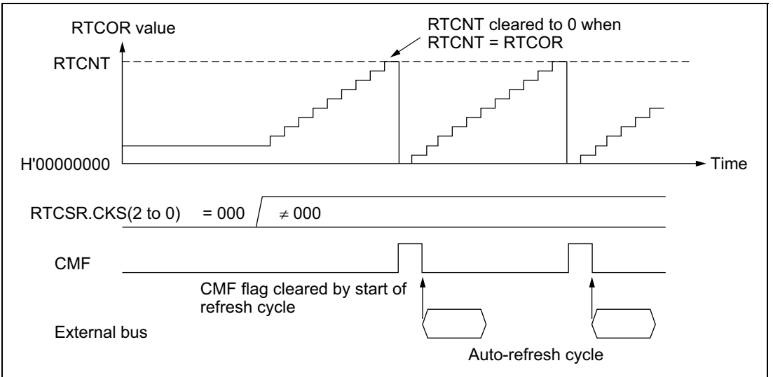
Figure 10.25 Auto-Refresh Operation
