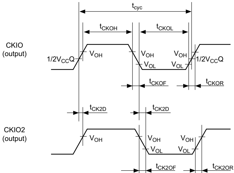
Figure 23.3 CKIO Clock Output Timing
