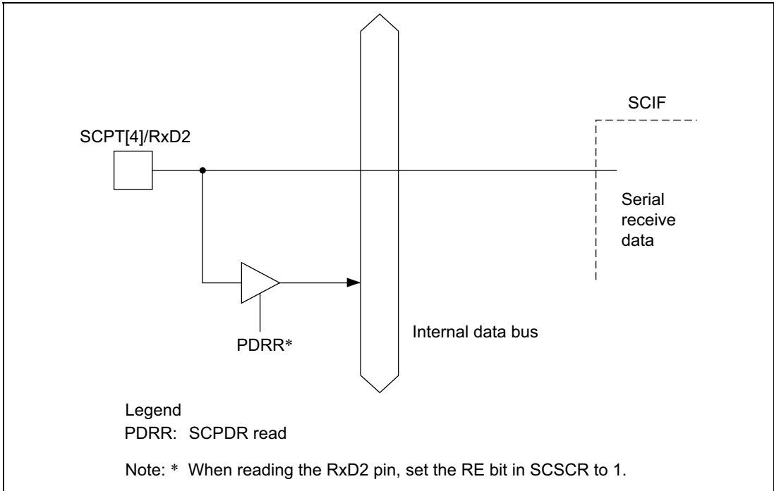
Figure 16.4 SCPT[4]/RxD2 Pin
