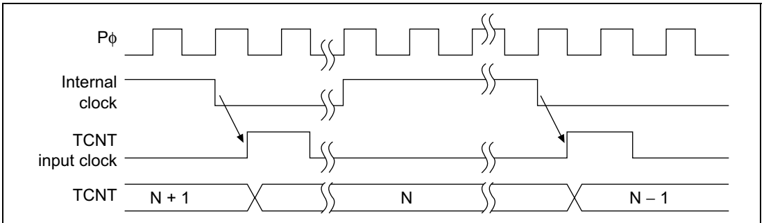
Figure 12.4 Count Timing when Operating on Internal Clock
