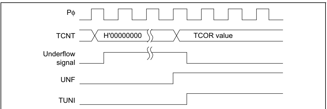
Figure 12.8 UNF Setting Timing
