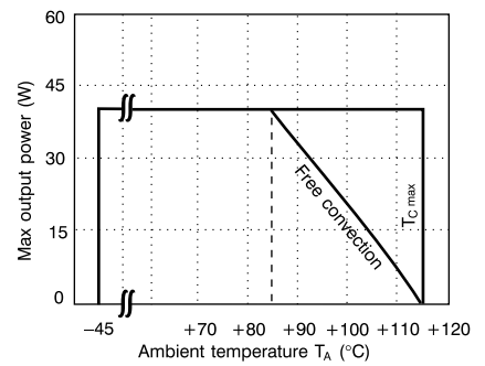
Power derating
