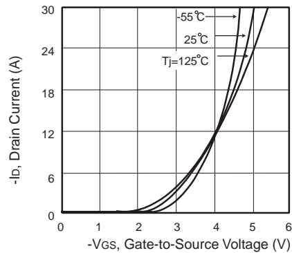
Figure 2. Transfer Characteristics
