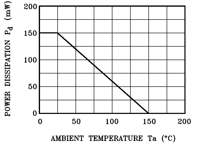
P_d - T_a
