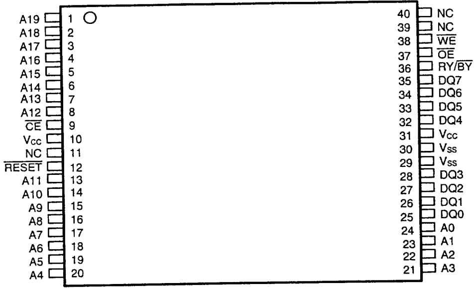
Standard TSOP
