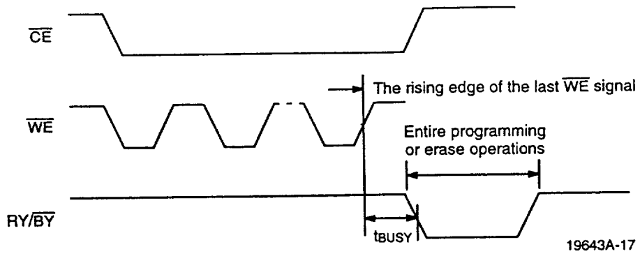
Figure 13. RY/\overline{BY} Timing Diagram During Program/Erase Operations
