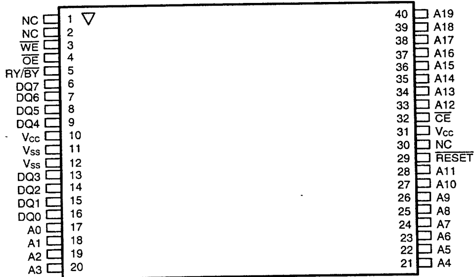
Reverse TSOP
