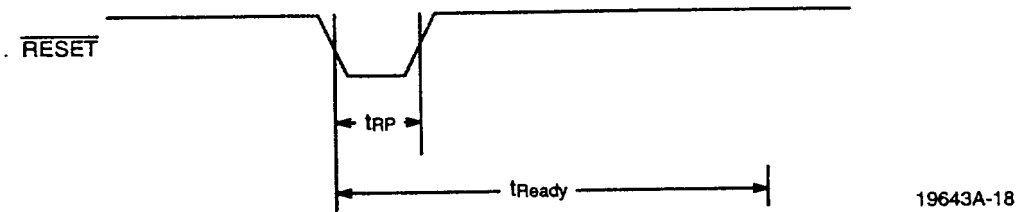
Figure 14. \overline{RESET} Timing Diagram
