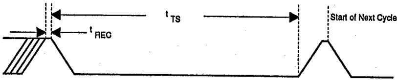
READ DATA TIME SLOTS Figure 3
