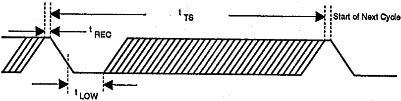
READ DATA TIME SLOTS Figure 3
