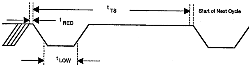
WRITE ONE TIME SLOT Figure 1
