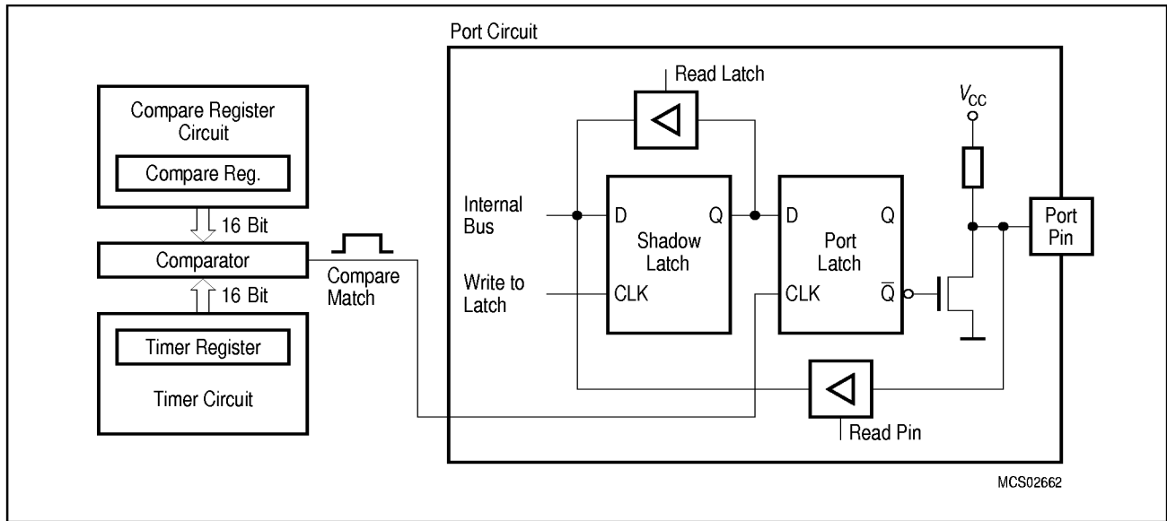
Figure 14 Compare Function in Compare Mode 1
