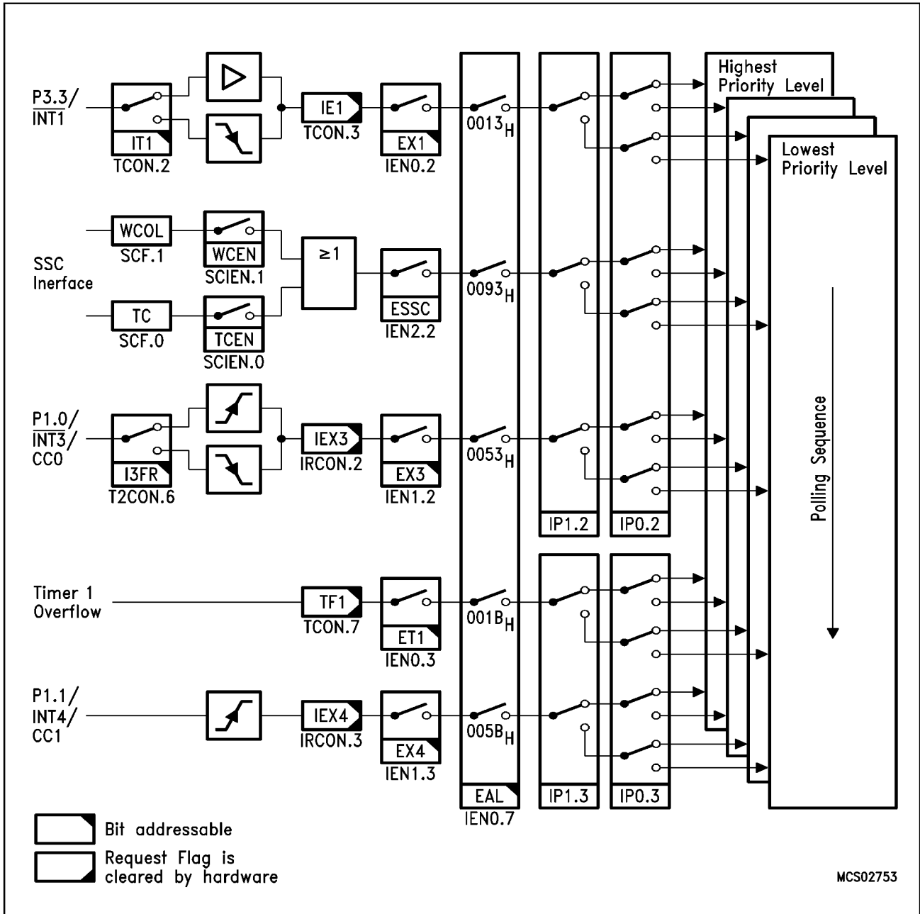
Figure 21 Interrupt Request Sources (Part 2)
