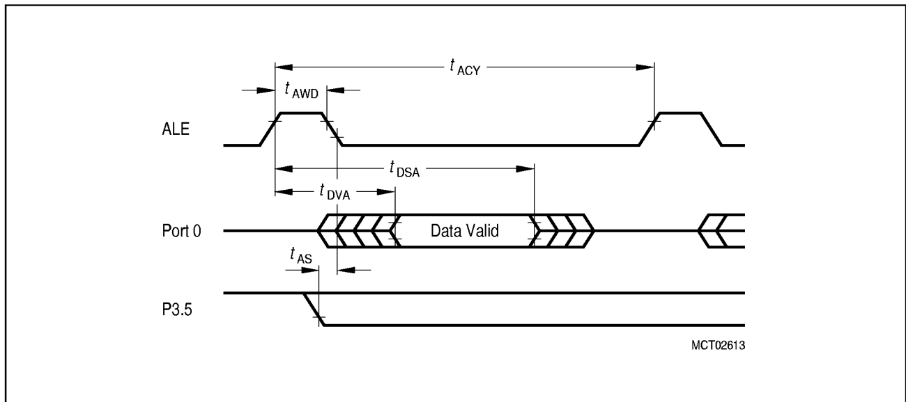
Figure 32 ROM Verification Mode 2
