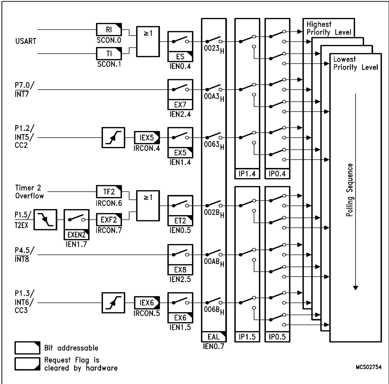
Figure 22 Interrupt Request Sources (Part 3)
