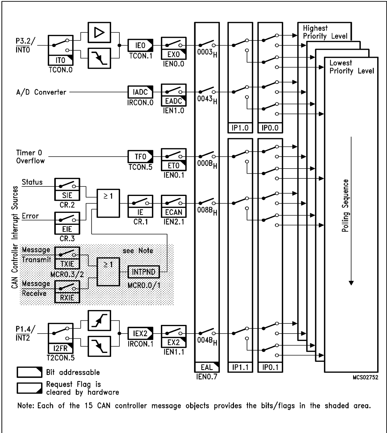
Figure 20 Interrupt Request Sources (Part 1)
