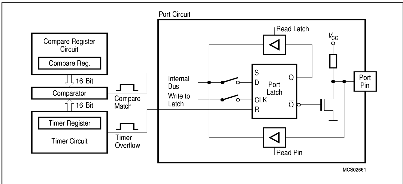
Figure 13 Port Latch in Compare Mode 0
