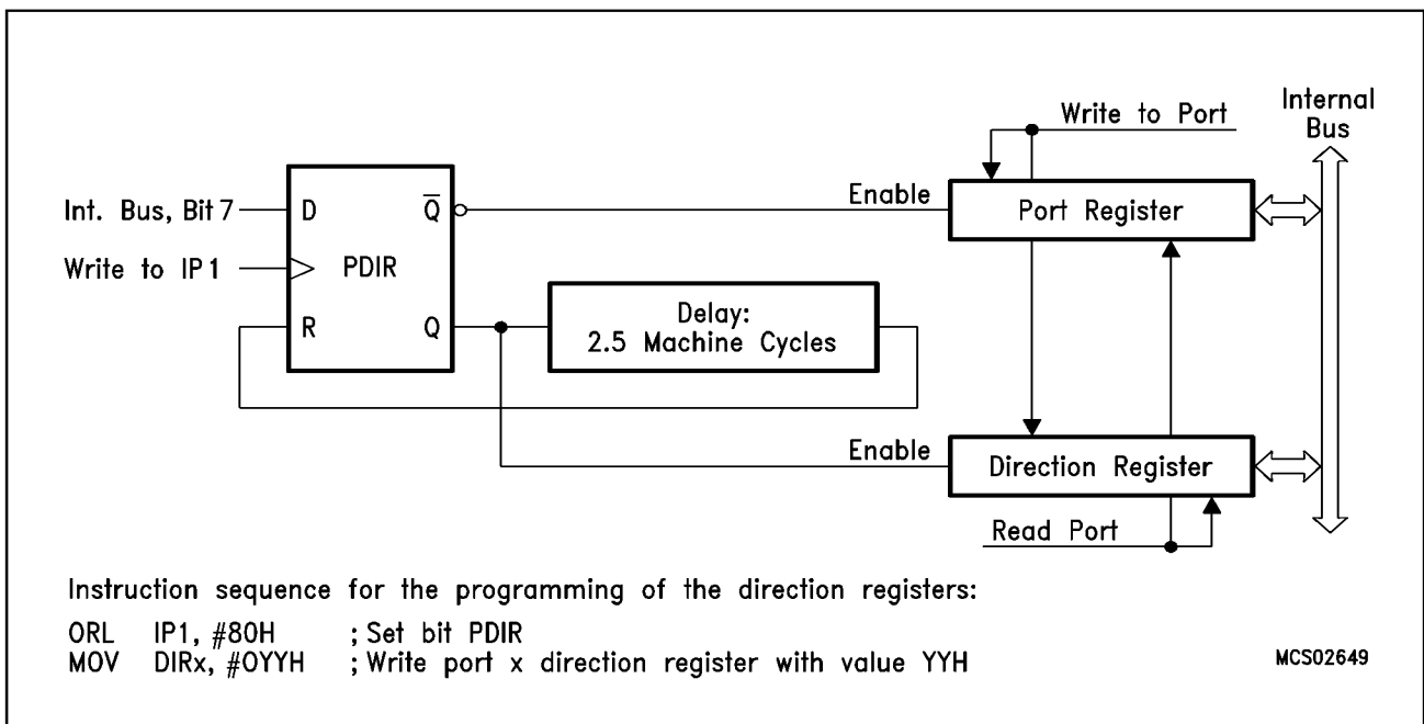
Figure 10 Port Register, Direction Register
