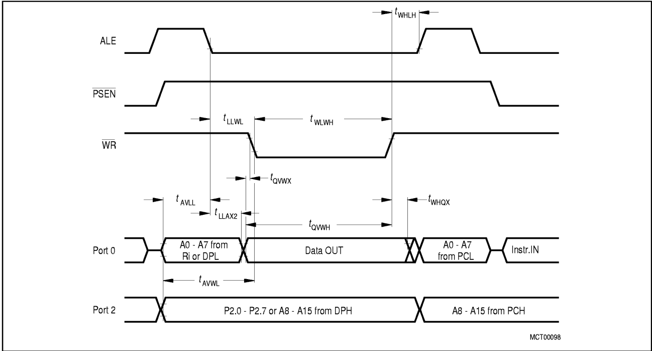
Figure 28 Data Memory Write Cycle
