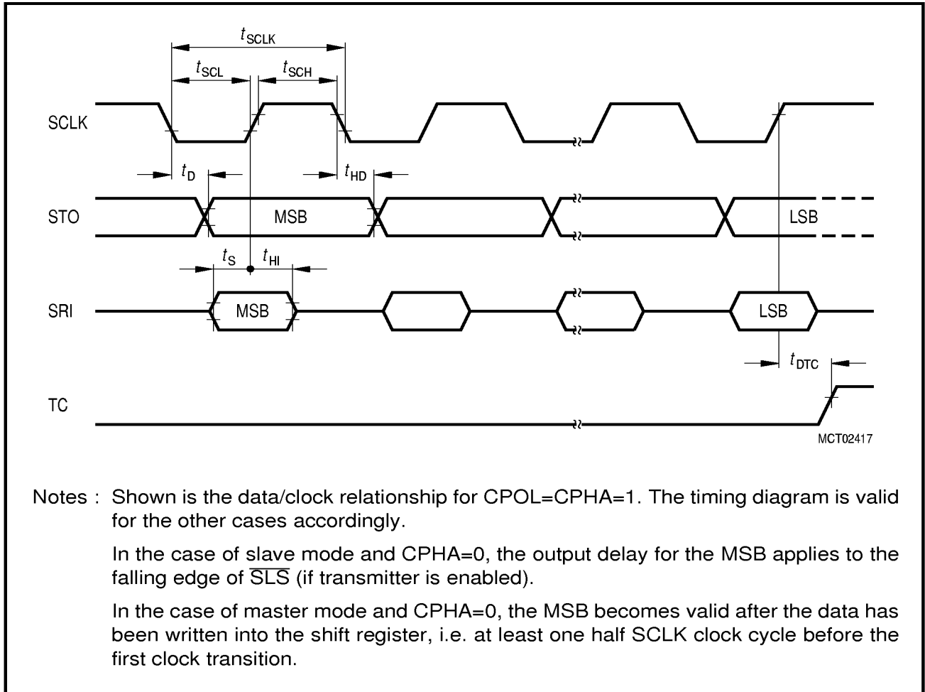
Figure 30 SSC Timing
