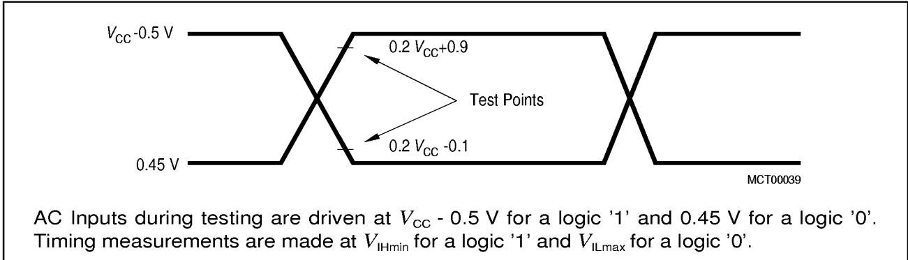
Figure 33 AC Testing: Input, Output Waveforms
