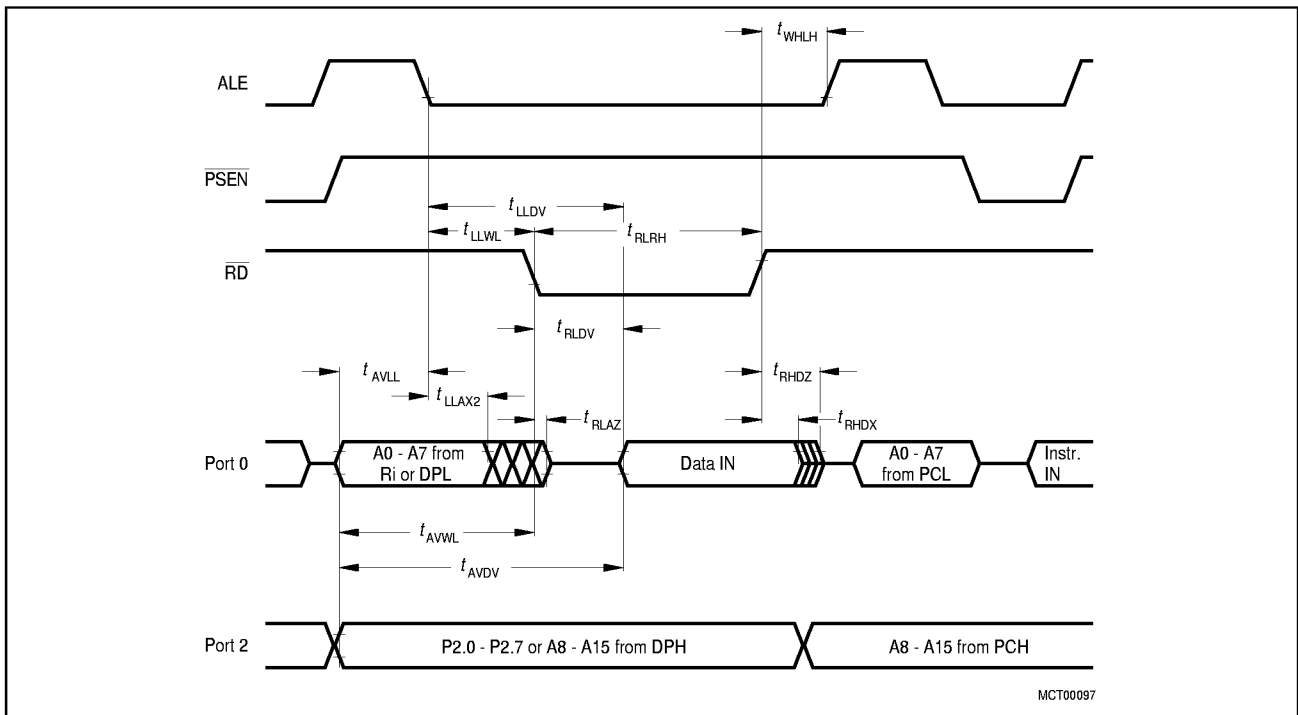
Figure 27 Data Memory Read Cycle
