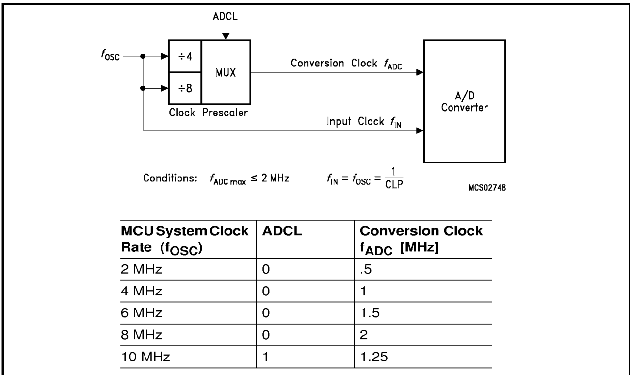
Figure 18 A/D Converter Clock Selection
