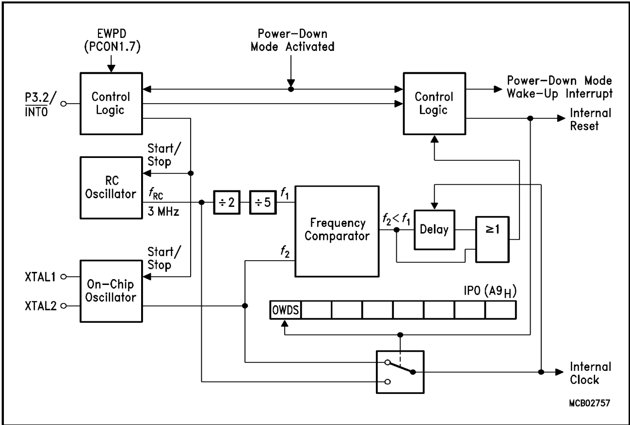
Figure 24 Block Diagram of the Oscillator Watchdog
