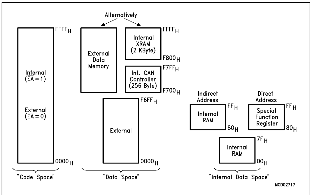
Figure 5 C515C Memory Map
