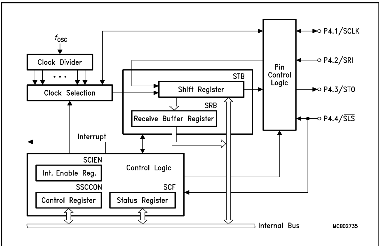
Figure 16 SSC Block Diagram
