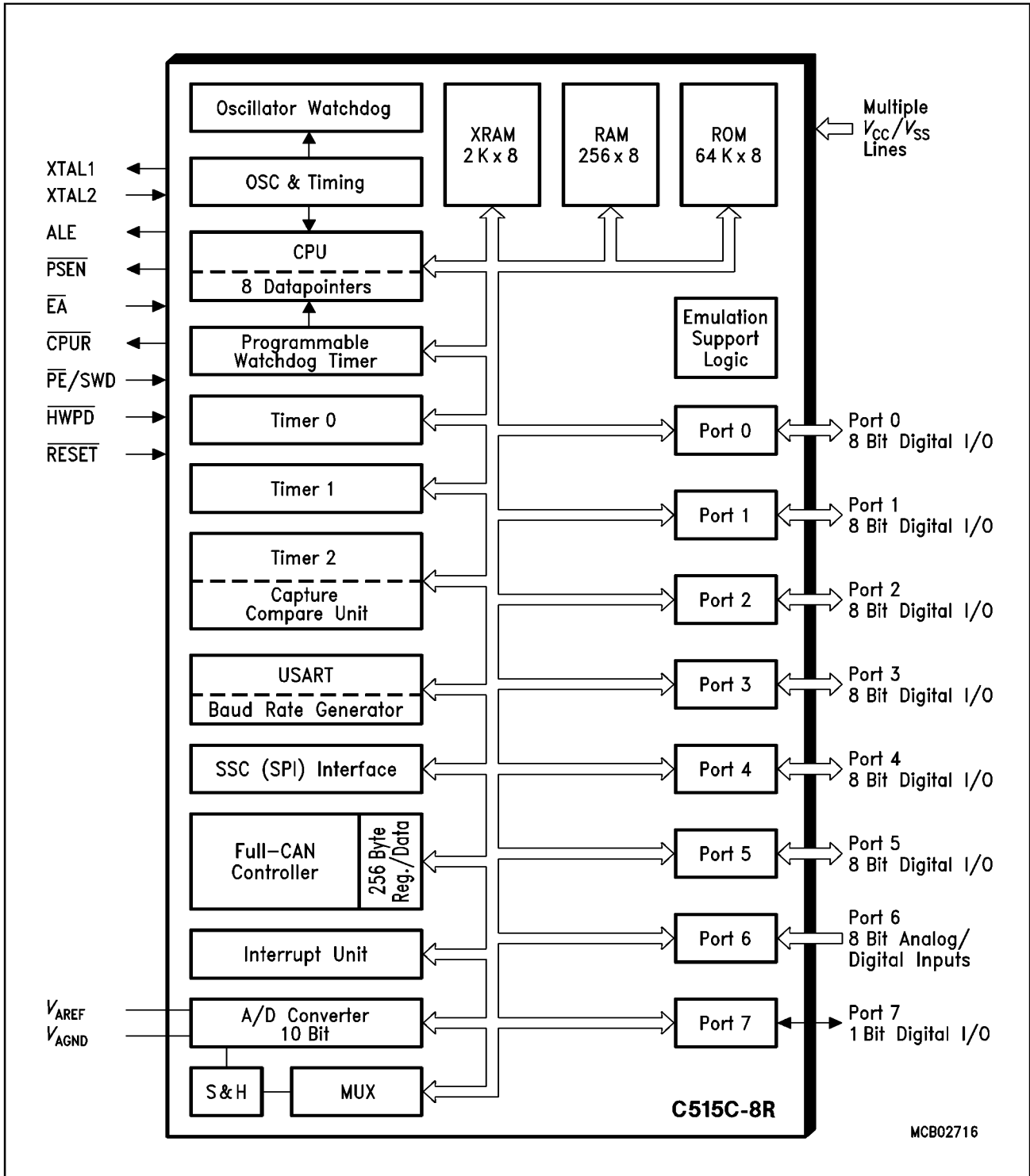
Figure 4 Block Diagram of the C515C
