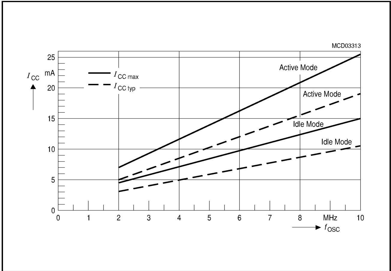
Figure 25 ICC Diagram
