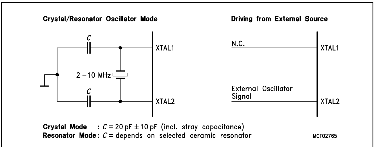
Figure 35 Recommended Oscillator Circuits for Crystal Oscillator
