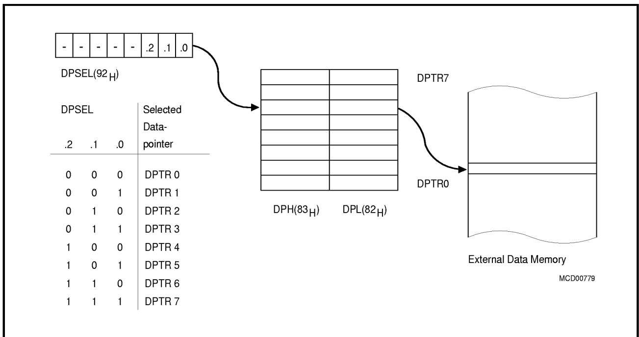
Figure 8 External Data Memory Addressing using Multiple Datapointers
