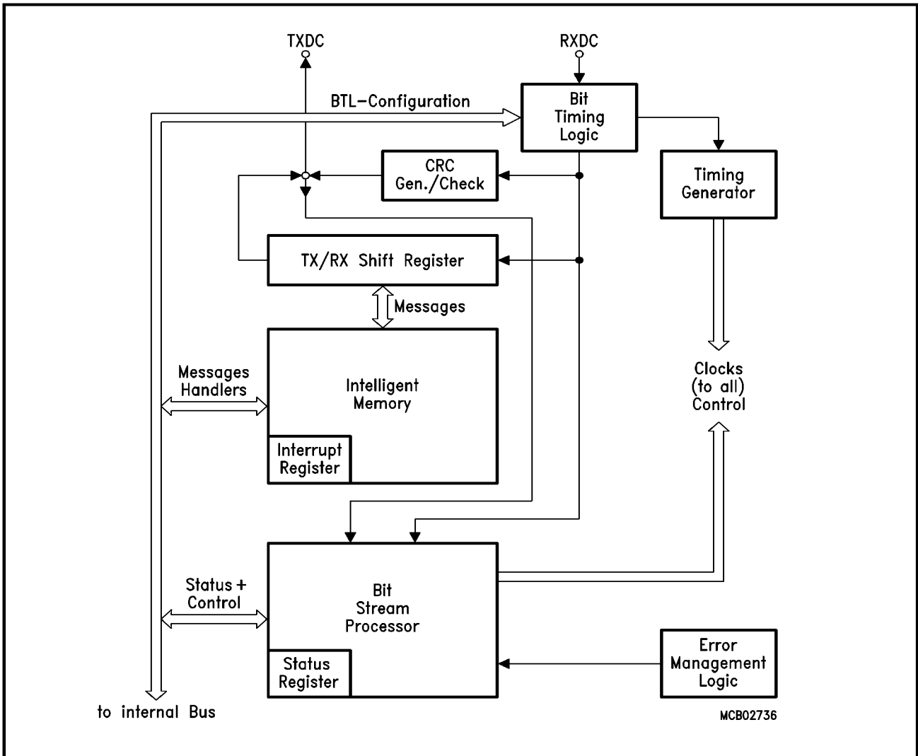
Figure 17 CAN Controller Block Diagram
