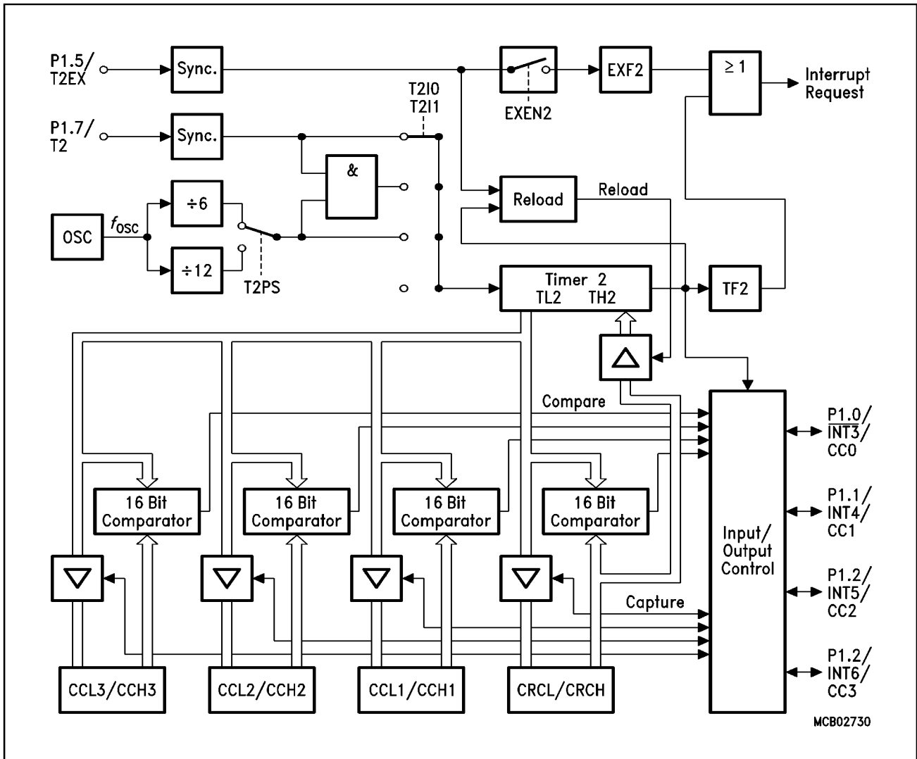
Figure 12 Timer 2 Block Diagram
