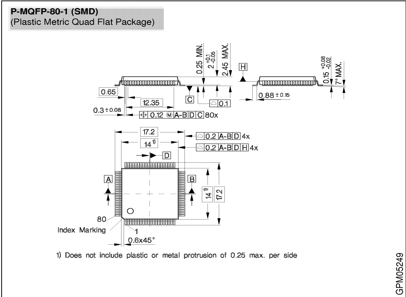
Figure 36 Package Outlines
