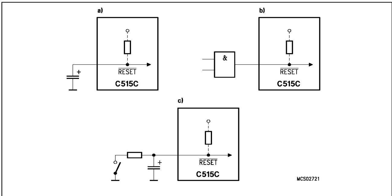
Figure 6 Reset Circuitries
