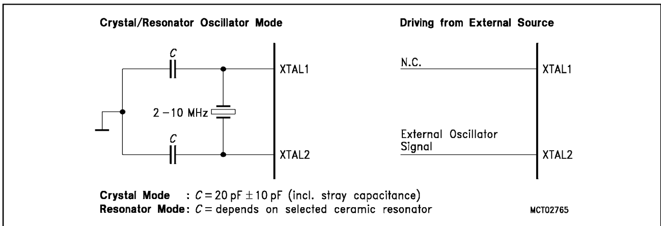
Figure 7 Recommended Oscillator Circuitries
