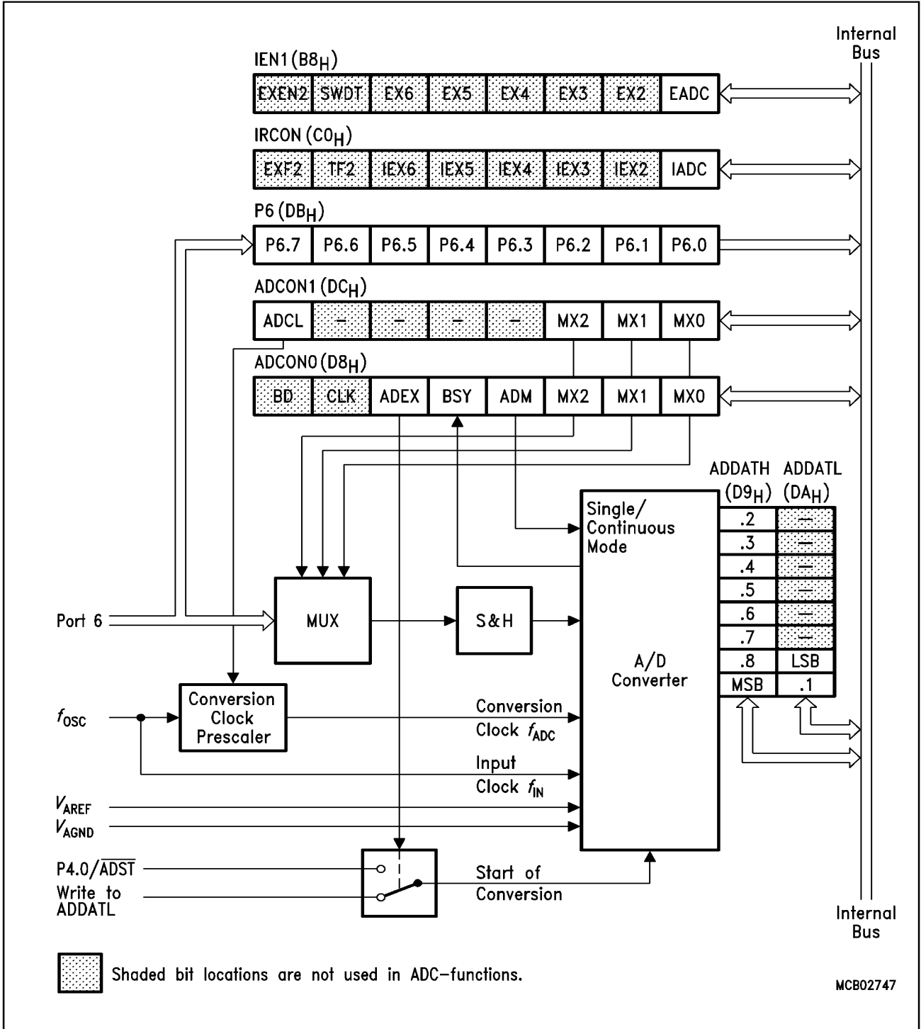
Figure 19 A/D Converter Block Diagram
