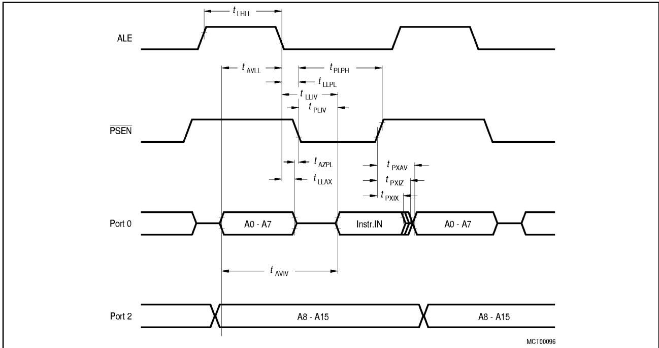
Figure 26 Program Memory Read Cycle
