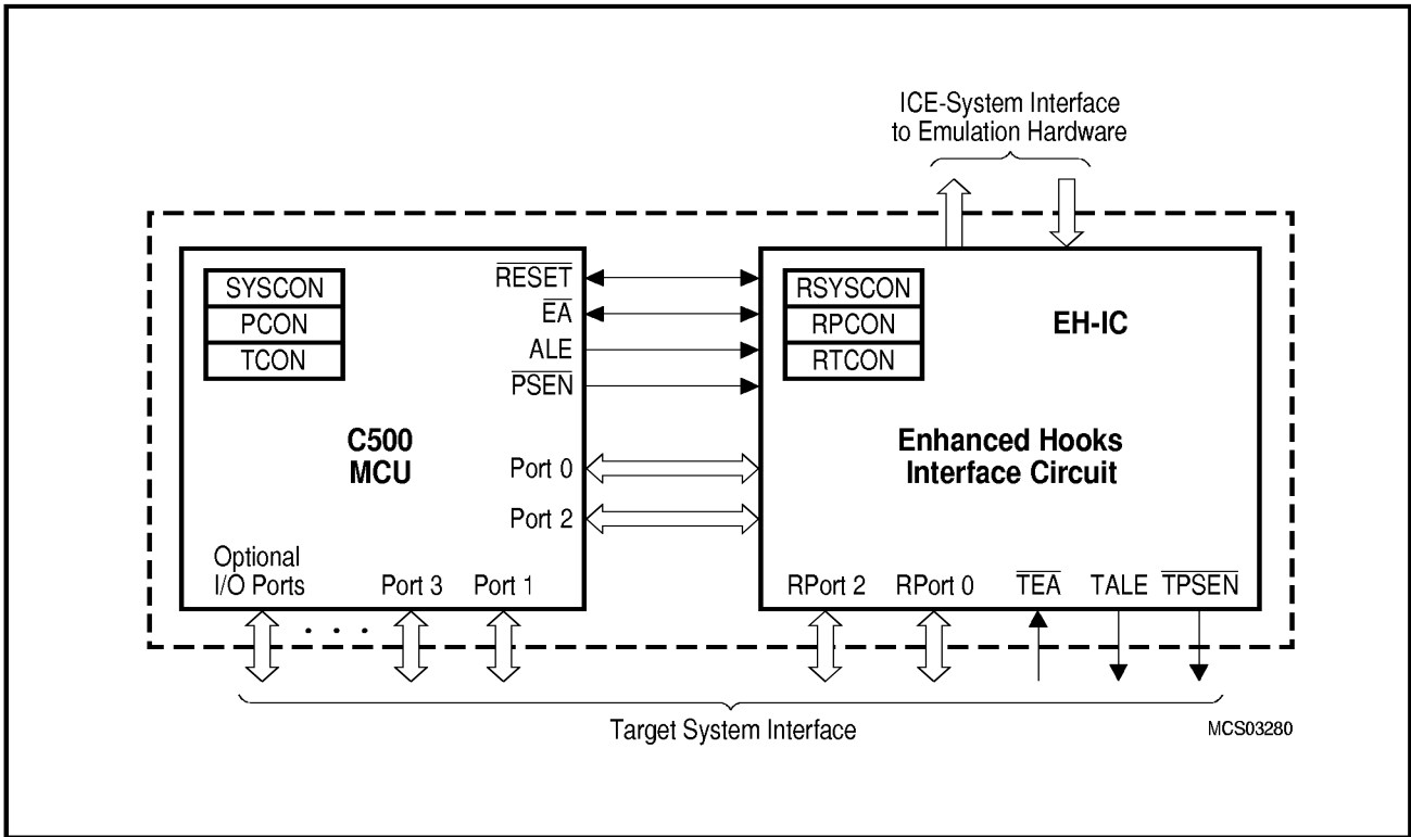
Figure 9 Basic C500 MCU Enhanced Hooks Concept Configuration
