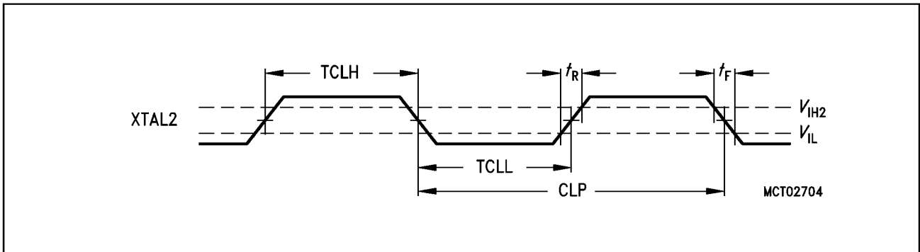
Figure 29 External Clock Drive at XTAL2
