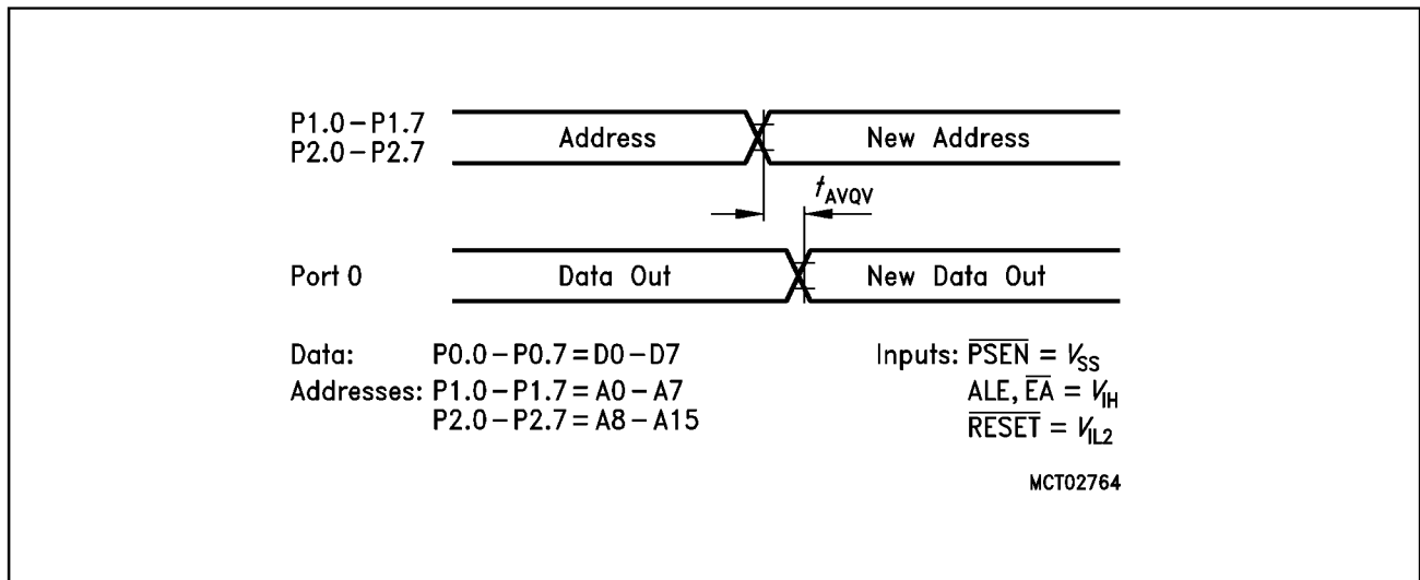
Figure 31 ROM Verification Mode 1
