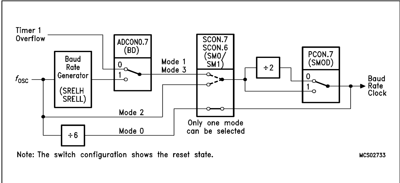
Figure 15 Block Diagram of Baud Rate Generation for the Serial Interface
