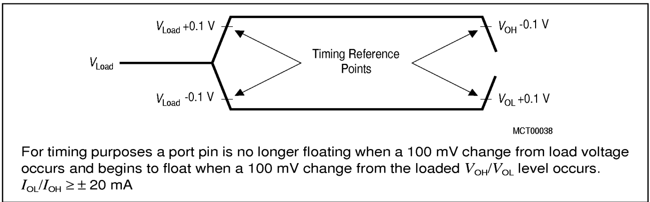
Figure 34 AC Testing : Float Waveforms
