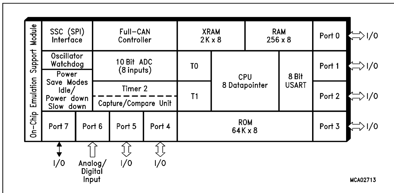
Figure 1 C515C Functional Units
