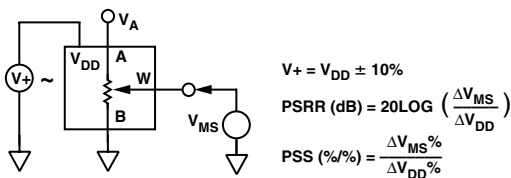
Test Circuit 4. Power Supply Sensitivity (PSS, PSRR)
