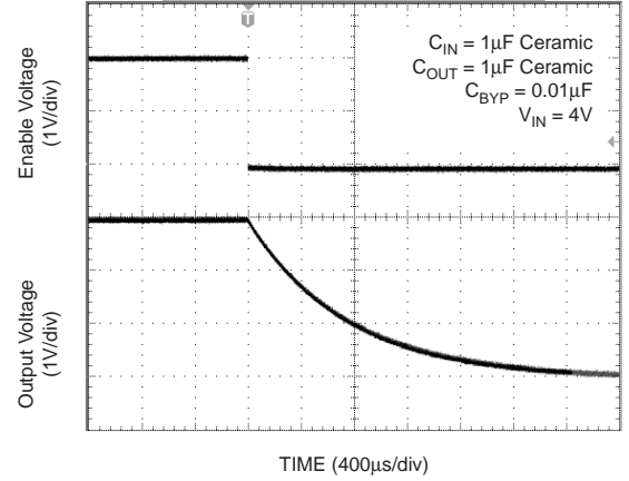
Shutdown Delay
