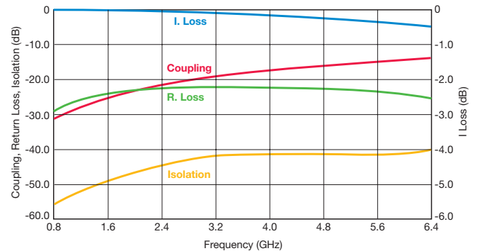
CP0402AxxxxFLTR
