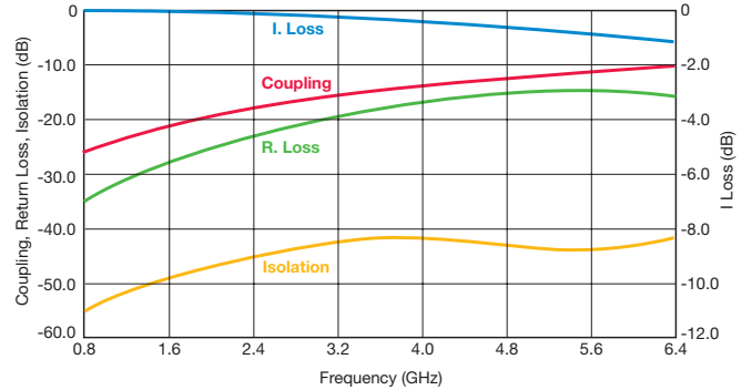
CP0402AxxxxELTR
