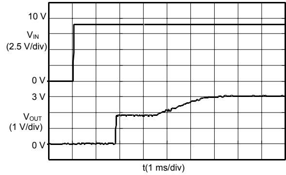
S-8520/1A30MC ( V_{IN} : 0 → 9.0 V)
