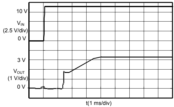
S-8520/1E33MC ( V_{IN} : 0 → 9.0 V)
