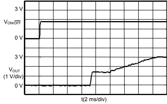
S-8520/1C30MC ( V_{IN} :9.0 V)
