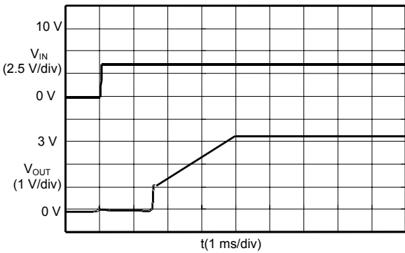
S-8520/1E33MC ( V_{IN} : 0 → 4.0 V)
