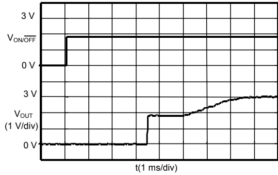
S-8520/1A30MC ( V_{IN} :9.0 V)
