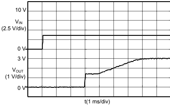
S-8520/1A30MC ( V_{IN} : 0 → 3.6 V)
