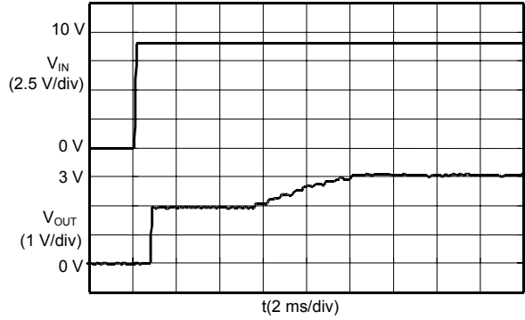
S-8520/1C30MC ( V_{IN} : 0 → 9.0 V)
