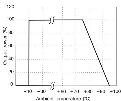
Power derating
