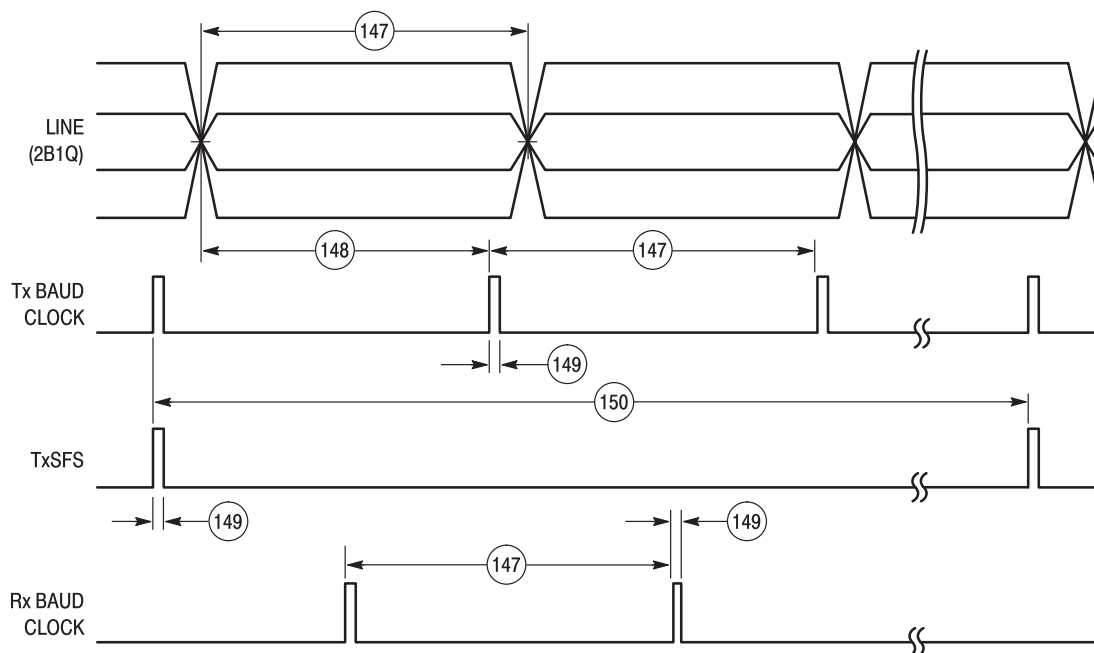
Figure 10–19. Baud Clock Timing
