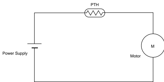
DC Motor Protection Circuit
