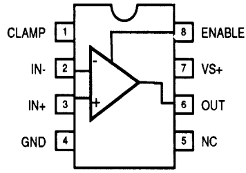
EL2157 (8-PIN SO, PDIP) TOP VIEW
