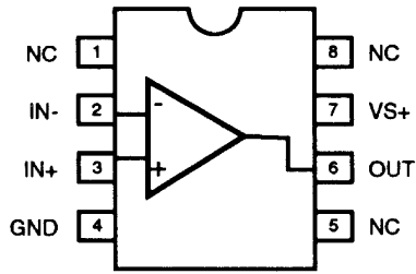
EL2150 (8-PIN SO, PDIP) TOP VIEW
