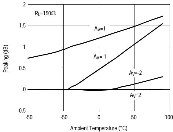
Peaking vs Temperature
