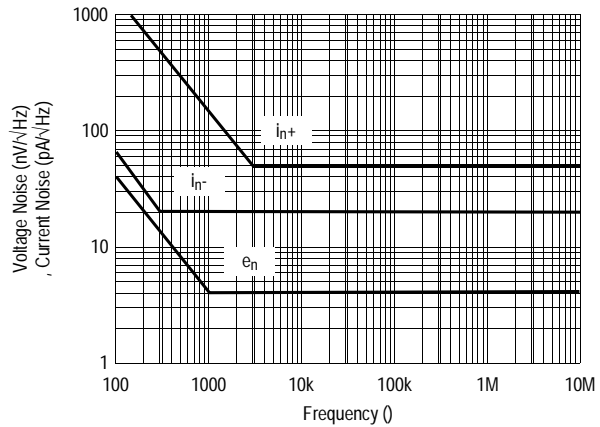
Voltage and Current Noise vs Frequency
