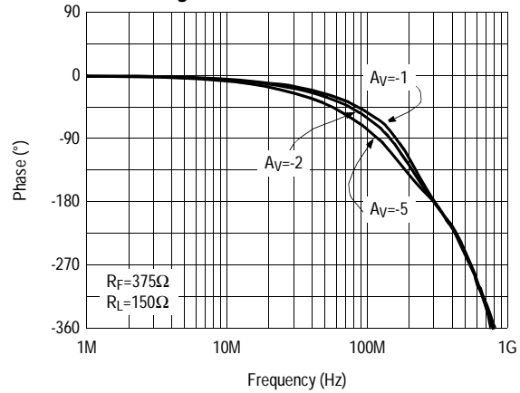
Inverting Frequency Response (Phase) SO8 Package
