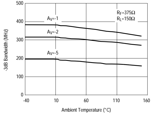
-3dB Bandwidth vs Temperature for Inverting Gains
