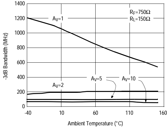
-3dB Bandwidth vs Temperature for Non-inverting Gains
