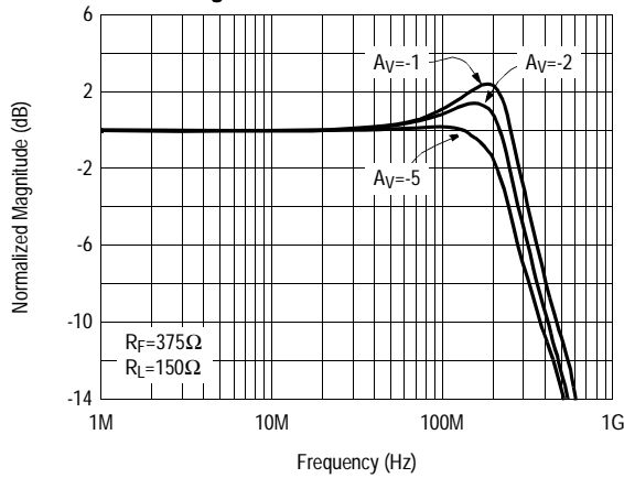
Inverting Frequency Response (Gain) SO8 Package
